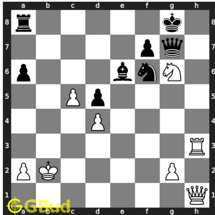
Figure 1.1: Solve this medium chess puzzle 0133. Mate in 2 moves @ https://gbud.in/g2cbq72
