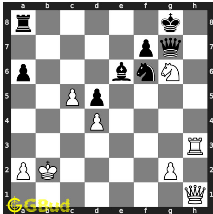
Figure 1.3: Initial board position of medium chess puzzle 0133
